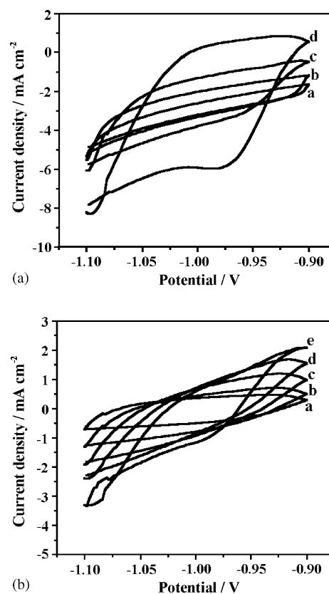
Fig. 1. Cyclic voltammograms obtained using porous Ni cell assemblies of (a) symmetric supercapacitor (porous Ni|KOH|porous Ni) at various scan rates of (a) 50 mV s -1 , (b) 100 mV s -1 , (c) 200 mV s -1 and (d) 500 mV s -1 and (b) asymmetric supercapacitor (porous Ni|KOH|activated carbon) at various scan rates such as (a) 25 mV s -1 , (b) 50 mV s -1 , (c) 100 mV s -1 , (d) 200 mV s -1 and (e) 500 mV s -1 in 6 M KOH aqueous solution.
