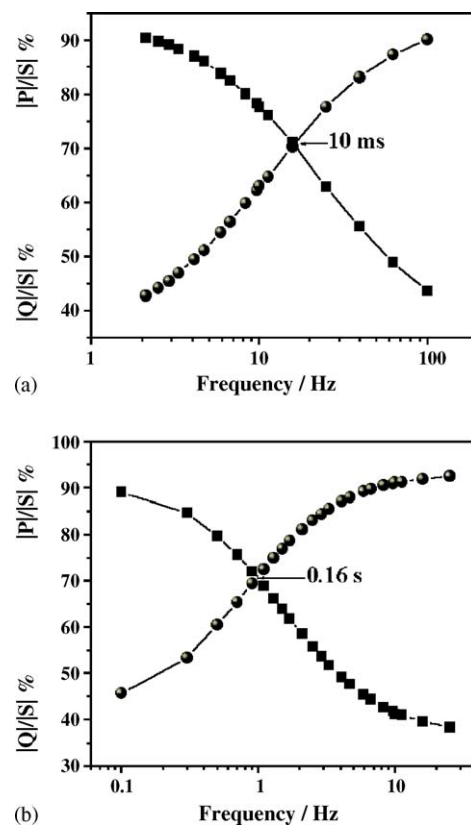
Fig. 7. Plots of normalized active power, |P|/|S| and reactive power |Q|/|S| vs. frequency (in logarithmic scale) for (a) symmetric and (b) asymmetric supercapacitor cell assemblies using the high surface area porous Ni as an electrode material.
