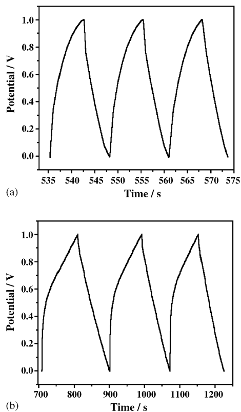
Fig. 9. Representative galvanostatic charge–discharge curves for the respective devices of (a) symmetric (porous Ni|KOH|porous Ni) and (b) asymmetric (porous Ni|KOH|activated carbon) supercapacitor cell assemblies based on the high surface area porous Ni as an electrode material in 6 \text{ M KOH} aqueous solution.
