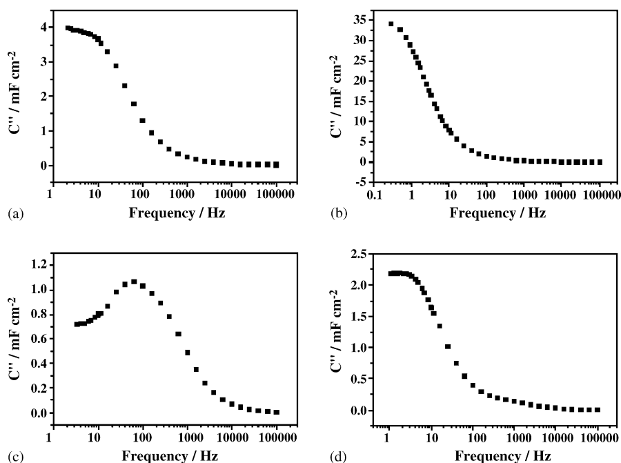
Fig. 6. The plots of imaginary part of the complex capacitance [ C''(\omega) ] with the frequency (in logarithmic scale) for (a) symmetric supercapacitor (porous Ni|KOH|porous Ni) and (b) asymmetric supercapacitor (porous Ni|KOH|activated carbon) based on the high surface area porous nickel electrode. (c) Symmetric supercapacitor (NiO|KOH|NiO) and (d) asymmetric supercapacitor (NiO|KOH|activated carbon) based on the nickel oxide electrode.
