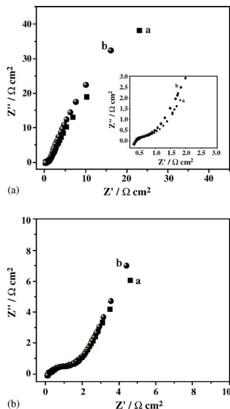
Fig. 4. Nyquist plots using high surface area porous Ni as an electrode material for (a) symmetric supercapacitor (porous Ni|KOH|porous Ni) at two different dc potentials of (a) -1.0 V and (b) -0.9 V and for (b) asymmetric supercapacitor (porous Ni|KOH|activated carbon) at two different dc potentials of (a) -1.0 V and (b) -0.9 V in 6 M KOH aqueous solution. Inset shows the expanded high frequency region of the same plot.
