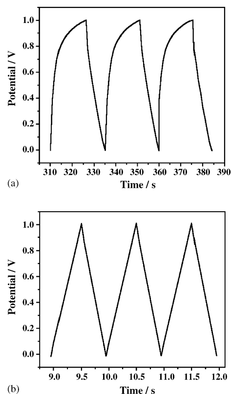
Fig. 10. Typical galvanostatic charge–discharge profiles of (a) symmetric (NiO|KOH|NiO) and (b) asymmetric (NiO|KOH|activated carbon) supercapacitor cell assemblies based on NiO as an electrode in 6 M KOH aqueous solution, respectively.
