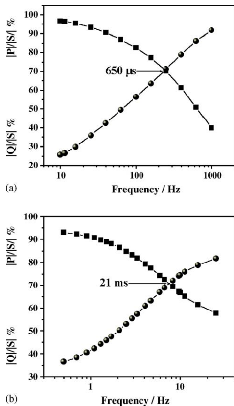
Fig. 8. Plots of normalized active power, |P|/|S| and reactive power |Q|/|S| vs. frequency (in logarithmic scale) for (a) symmetric and (b) asymmetric supercapacitor cell assemblies using NiO obtained from the electrochemical oxidation of porous Ni as an electrode material.
