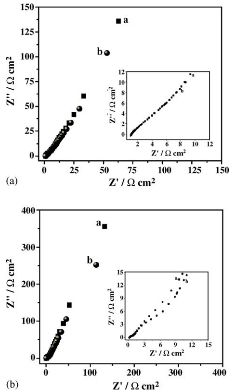
Fig. 5. Typical impedance (Nyquist) plots using NiO obtained from the porous Ni as an electrode material in 6M KOH aqueous solution for (a) symmetric supercapacitor (NiO|KOH|NiO) at dc potentials of (a) 0 V and (b) 0.1 V and (b) asymmetric supercapacitor (NiO|KOH|activated carbon) at dc potentials of (a) 0 V and (b) 0.1 V. Inset shows the zoomed portion of the same plot at high frequency region.
