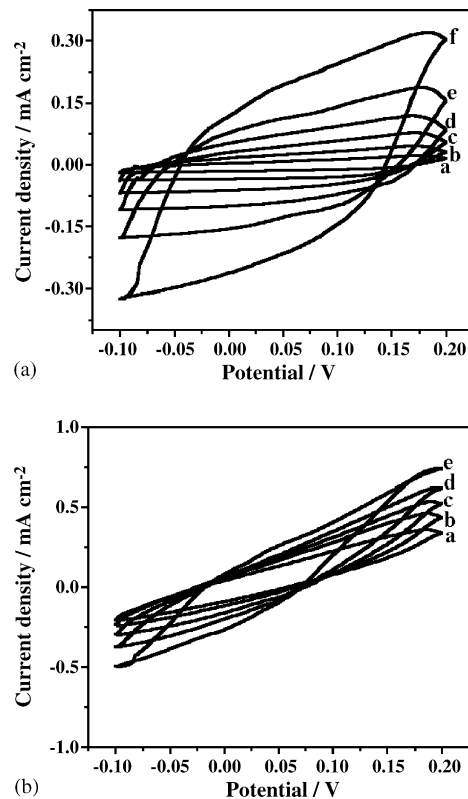
Fig. 2. Cyclic voltammograms obtained using NiO cell assemblies of (a) symmetric supercapacitor ( \text{NiO}|\text{KOH}|\text{NiO} ) at different scan rates such as (a) 10 \text{ mV s}^{-1} , (b) 25 \text{ mV s}^{-1} , (c) 50 \text{ mV s}^{-1} , (d) 100 \text{ mV s}^{-1} , (e) 200 \text{ mV s}^{-1} and (f) 500 \text{ mV s}^{-1} and (b) asymmetric supercapacitor ( \text{NiO}|\text{KOH}|\text{activated carbon} ) at different scan rates of (a) 25 \text{ mV s}^{-1} , (b) 50 \text{ mV s}^{-1} , (c) 100 \text{ mV s}^{-1} , (d) 200 \text{ mV s}^{-1} and (e) 500 \text{ mV s}^{-1} in 6 M KOH aqueous solution.
