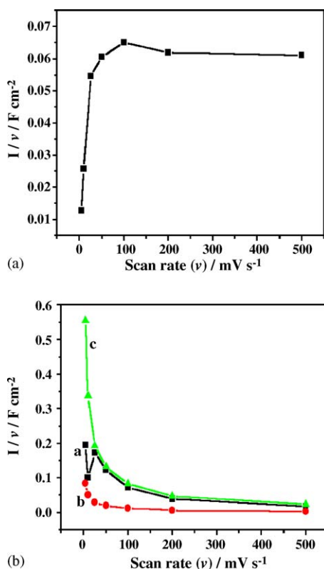
Fig. 3. Variation of I/\nu with different scan rates used for the capacitance measurement using cyclic voltammetry for (a) symmetric supercapacitor of high surface area porous nickel (porous Ni|KOH|porous Ni). (b) Similar plots for the other cell assemblies namely (a) asymmetric supercapacitor based on the porous nickel electrode (porous Ni|KOH|activated carbon), (b) symmetric supercapacitor (NiO|KOH|NiO) and (c) asymmetric supercapacitor (NiO|KOH|activated carbon) based on nickel oxide electrode.
